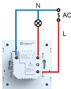
Connection 2: With neutral wire
