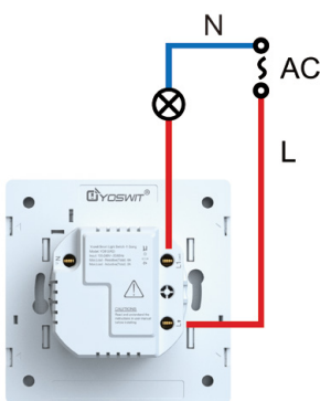
Connection 1: Without neutral wire
